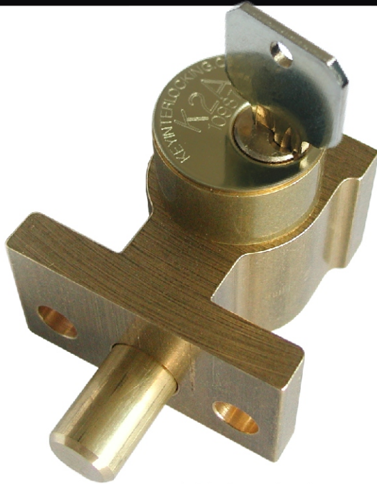
VB Interlock (bolt left)
