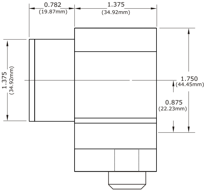
VB Interlock (bolt left)
